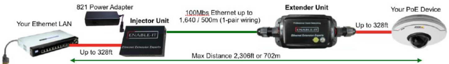
821WP Outdoor PoE Extender
